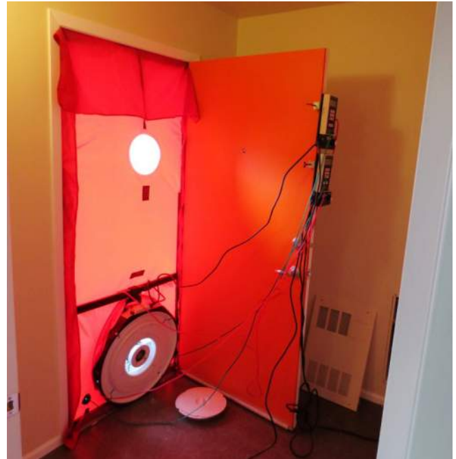
Typical blower door system installed in door frame for whole building airtightness testing.
