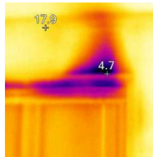
Infrared Thermography indicating air leakage at a window head (left), and showing a cold bathroom fan (right).
