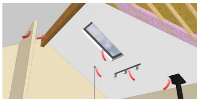
Cathedral ceiling air sealing locations.
