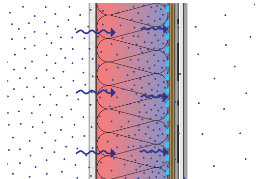
Potential condensation caused by vapour diffusion could be exacerbated by increased interior insulation, creating colder surface temperatures at the exterior enclosure elements.
