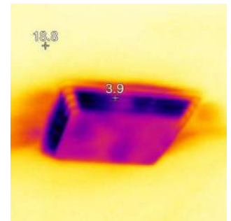
Infrared Thermography indicating air leakage at a window head (left), and showing a cold bathroom fan (right).
