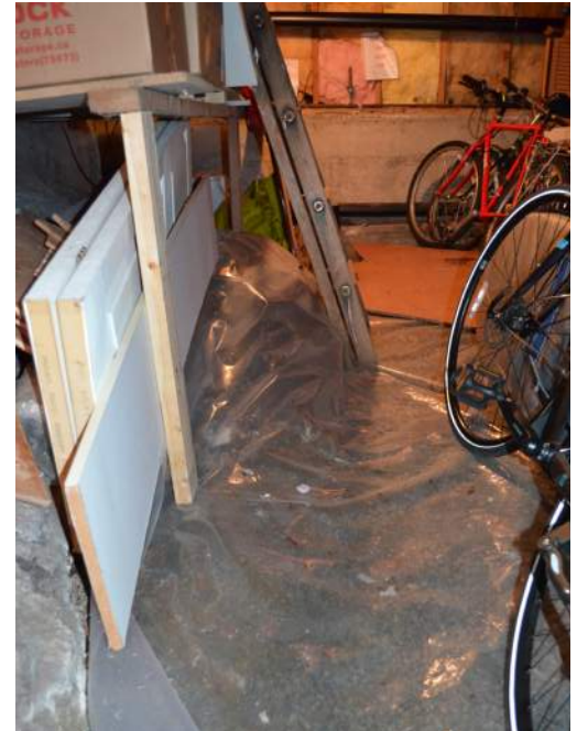
Certain floor conditions are difficult and impractical to air seal. Here a polyethylene sheet has been placed on top of the gravel and bedrock floor to reduce vapour drive into the crawlspace. The polyethylene in this frequently used basement will most likely be damaged.
