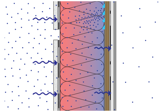
Potential condensation caused by air leakage through the enclosure assembly presents a risk to the assembly's durability.
