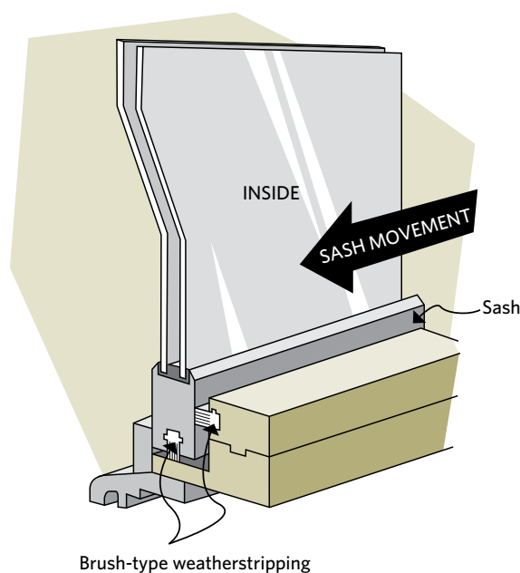
Figure 8-6 Brush weatherstripping on a sliding window
